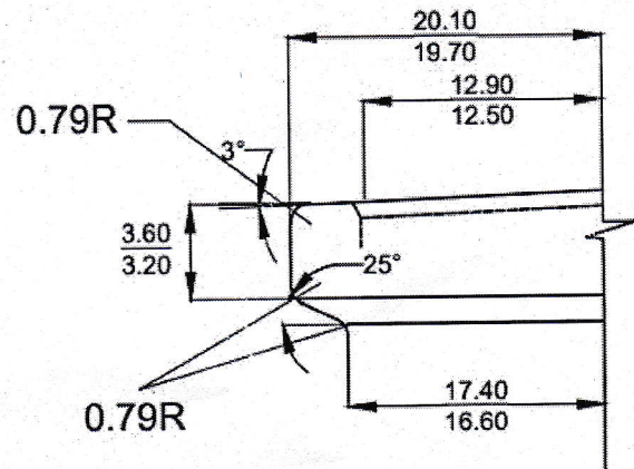
NECK FINISH DETAIL
